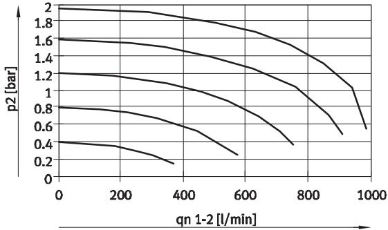
VPPM-8TA-...-0L2H-... (2 bar)
