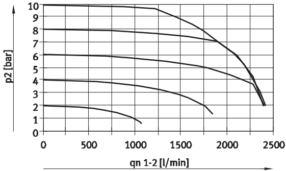
VPPM-8TA-...-0L10H-... (10 bar)
