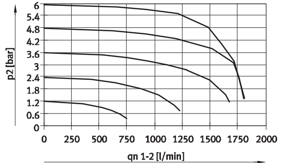
VPPM-8TA-...-0L6H-... (6 bar)
